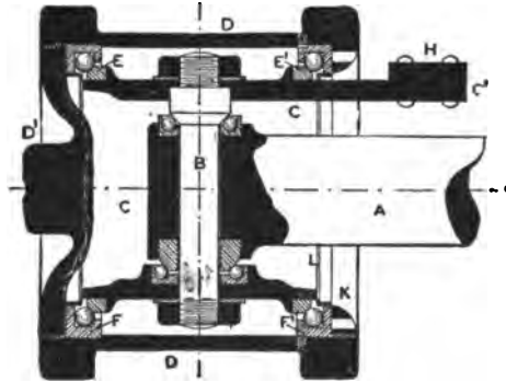
FIG. 32.—Pivoted Steering Hub used on the Riker Carriages. A is the axle shaft; B, the pivot connecting A to the tubular swinging hub, C. E and E' are circular cones which bear on the balls mounted in the ball races, F and F', thus permitting the hub D to rotate independently on the inner tube, C. The steering arm, H, attached to C turns both C and D on the pivot, B.
